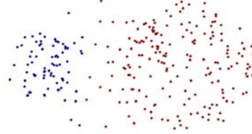
Two Clusters
