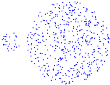
Original Points
