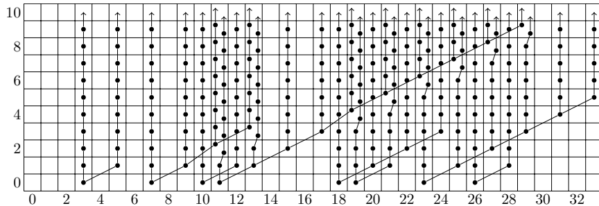
FIGURE 3. The v_0 -Bockstein spectral sequence converging to \overline{\mathrm{T}\mathrm{H}\mathrm{H}}_*(ku)
