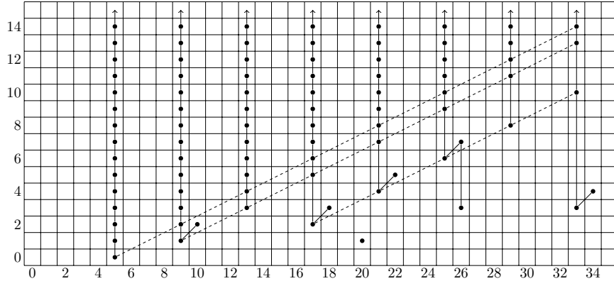
FIGURE 5. \overline{\mathrm{T}\mathrm{H}\mathrm{H}}_*(ko) through degree 34
