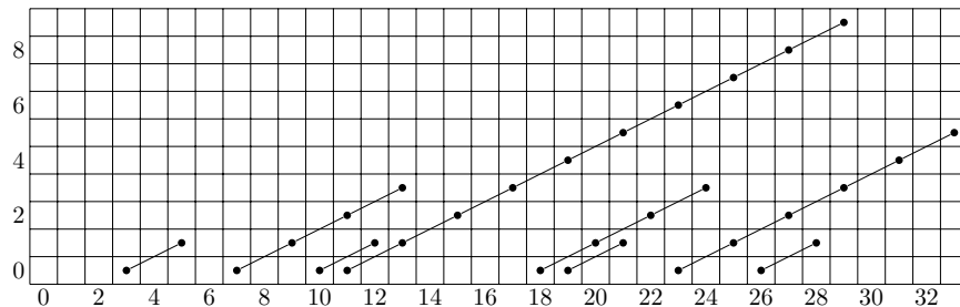
FIGURE 2. The homotopy of \overline{\mathrm{THH}}(ku; k(1))
