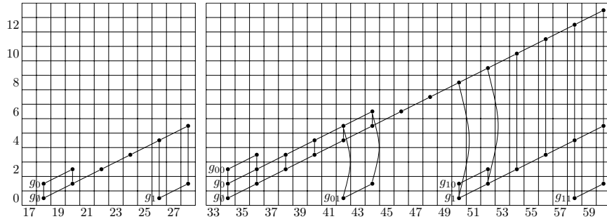
FIGURE 1. The torsion in degrees 18 through 60 for p = 2
