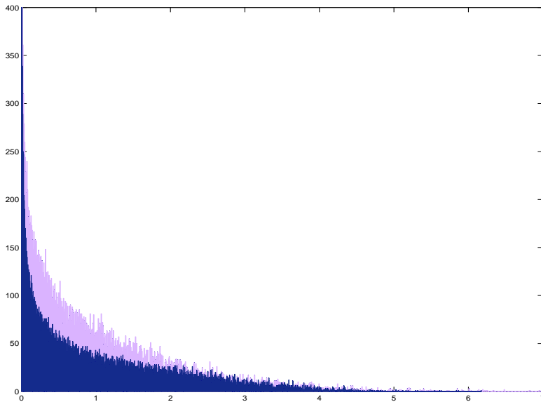
Figure 3: Histograms for empirical spectral distribution for 50 realizations of (1/n)HH' with N(0, 1) entries where H is a 500 \times 500 Hankel matrix with symmetric link function (color: light violet) and asymmetric link function (color: deep blue).
