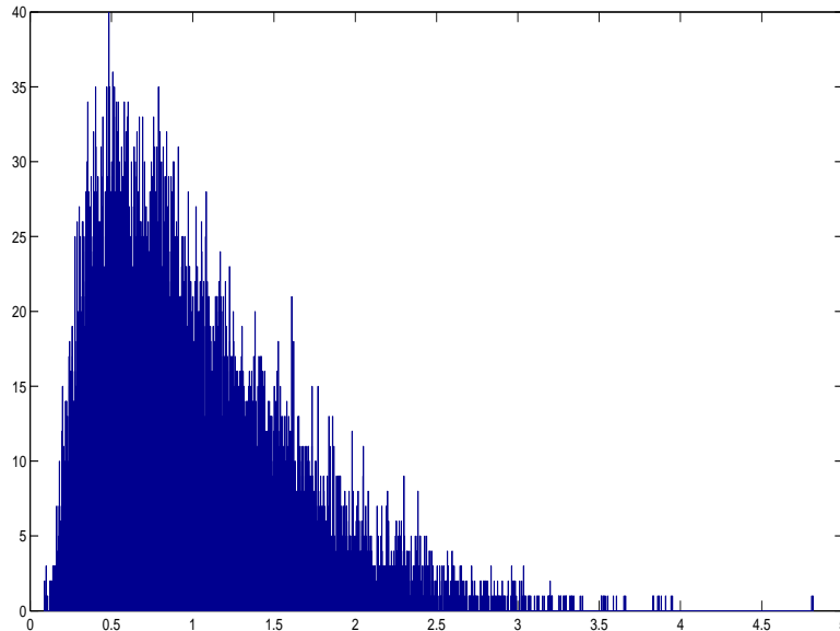
Figure 1: Histogram for empirical spectral distribution for 50 realizations of (1/n)TT' with U(-\sqrt{3}, \sqrt{3}) entries where T is a 300 \times 900 asymmetric Toeplitz matrix.
