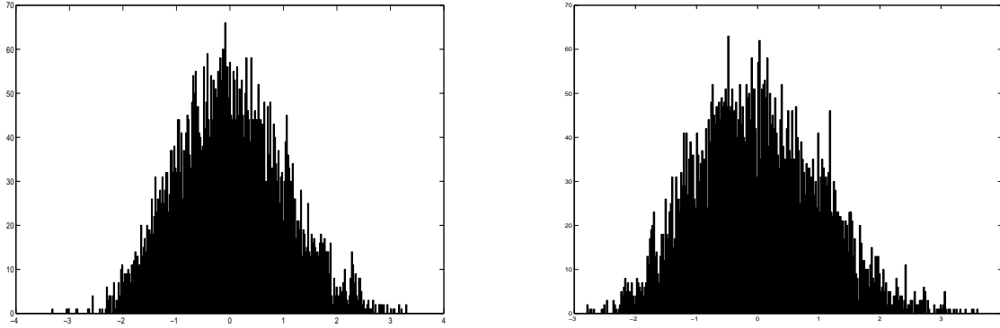
Figure 2: Histograms for empirical spectral distribution for 30 realizations of \frac{1}{\sqrt{np}}(TT' - nI) with N(0, 1) entries where T is a 200 \times 20000 Toeplitz matrix with asymmetric link function (left) and symmetric link function (right).
