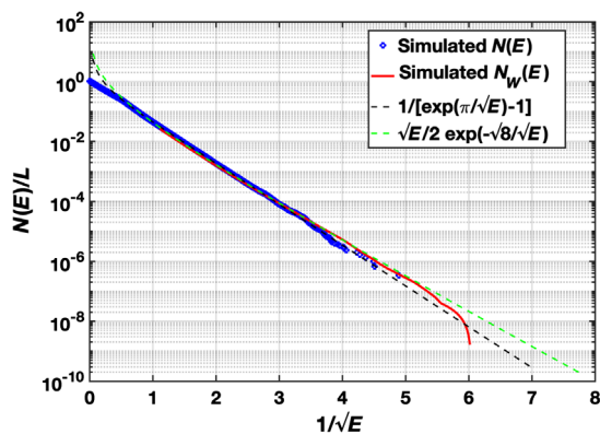
FIG. 1. Counting functions N(E) and N_W(E) computed on an interval of length L = 3.10^6 for \rho = 1 , superimposed with the corresponding predicted analytical formulas.
