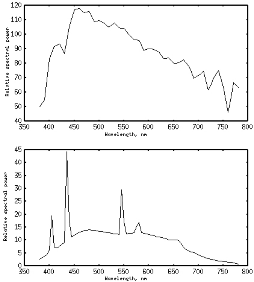
Figure 3. Spectral energy distributions for daylight (top) and a broad-band fluorescent light bulb(bottom).
