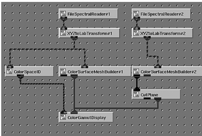
Figure 12. The gamut visualization application used to create the visualization of Figure 11.
