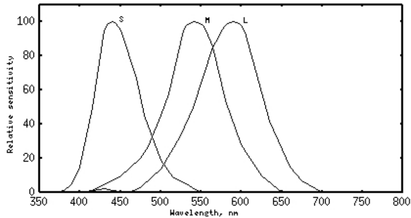
Figure 4. Approximation of the spectral curves of the sensitivities of the short, medium, and long wavelength receptors of the human eye. Curves are plotted short, medium, and long, left to right.
