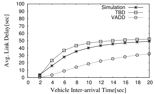
Figure 4. Link Delay Comparison for Model Validation
