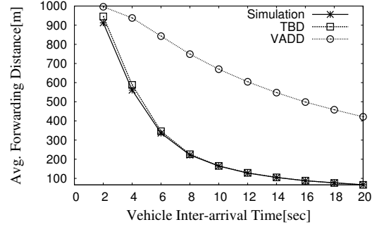
Figure 3. Validation and Comparison of Analytical Models
