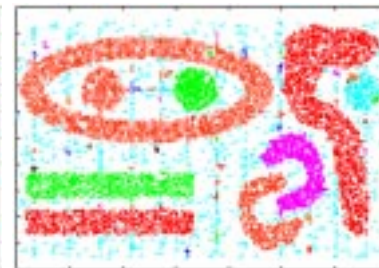
(h) DS4: Eps=6.2, MinPts=4
