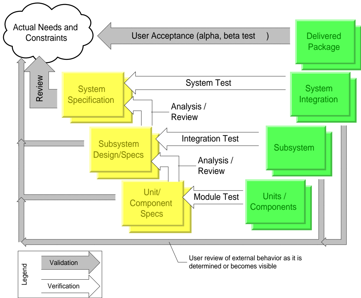
Figure 2.1: Validation activities check work products against actual user requirements, while verification activities check consistency of work products.
