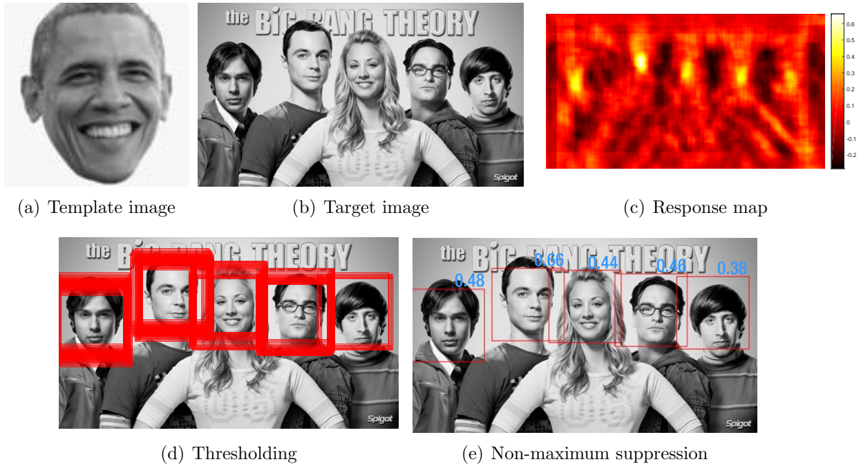
Figure 6: You will use (a) a single template image to detect faces in (b) the target image using HOG descriptors. (c) HOG descriptors from the template and target image patches can be compared by using the measure of normalized cross-correlation (NCC). (d) Thresholding on NCC score will produce many overlapping bounding boxes. (e) Correct bounding boxes for faces can be obtained by using non-maximum suppression.
