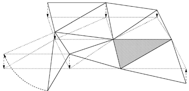
Fig. 4. A diagrammatic illustration of the flattening process. The normal of the gray-shaded triangle defines the plane into which the remaining triangles in the patch are projected. The union of these triangles defines the area across which the texture will be synthesized. Neighboring triangles from the adjacent patches are rotated (to minimize projective distortion) into the plane so that any texture already present in these triangles can provide boundary conditions for the texture synthesis, in order to enable the achievement of a seamless final result.
