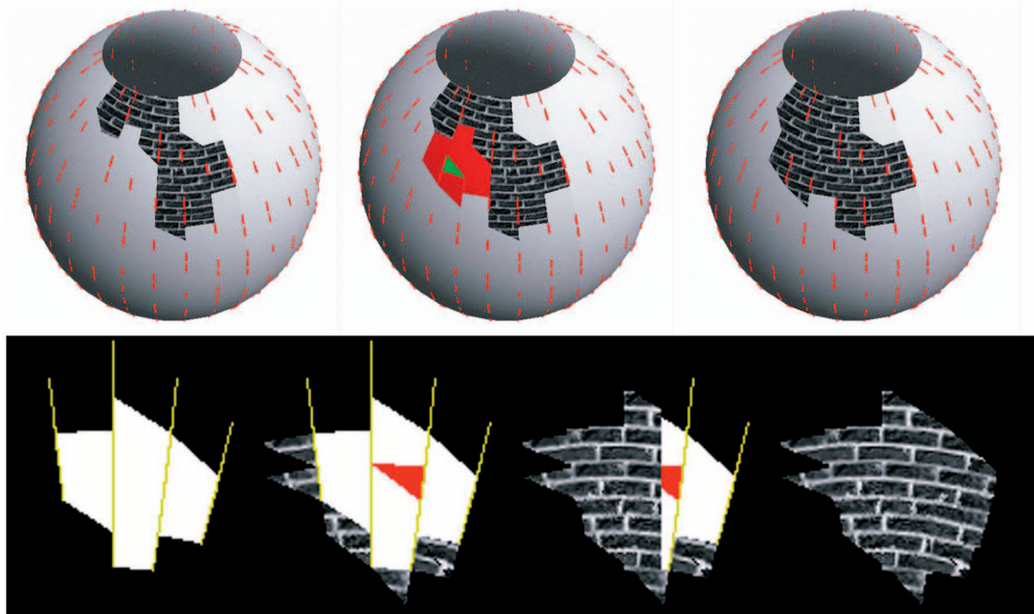
Fig. 6. A step-by-step illustration of the basic process of our method. Upper row: The identification of the patch to be synthesized and the synthesis result. Lower row (from left to right): The planar projection of the patch; the boundary conditions provided by the neighboring textured triangles rotated into the plane of the patch; midway through the texture synthesis process (synthesis is proceeding from left to right); the complete synthesized patch.
