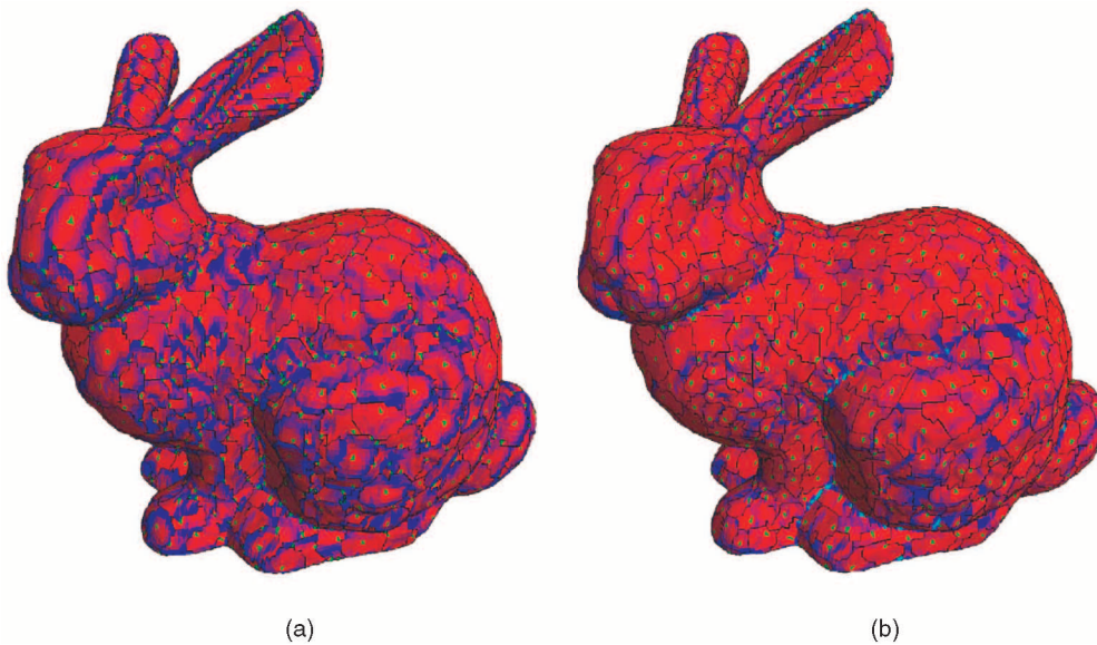
Fig. 3. The partitioned bunny, after the first stage of our “greedy” splitting algorithm (a) and after iterative refinement (b), which decreased the number of patches from 988 to 699. Patch boundaries are outlined in black on each model. The green triangles are the seed triangles, which also define the reference plane for each patch. Triangles whose normal directions differ by less than 18 degrees from the direction of the normal to the reference plane, corresponding to a 5 percent error in the linear projection, are colored red. Triangles up to 25 degrees out of alignment with the reference plane for their patch, corresponding to a 10 percent error in the projection, are colored blue. Triangles rotated more than 25 degrees from the reference plane (> 10 percent error) are colored cyan.
