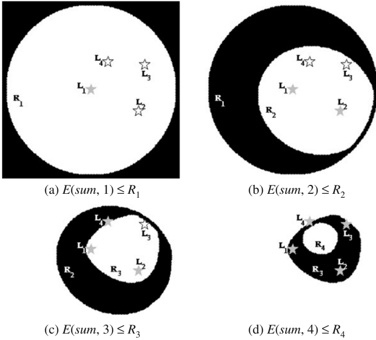
Fig. 7 Progressive reduction of P-CANN search space. The silver stars represent the foci of the locus of E(sum, i) \leq R_i
