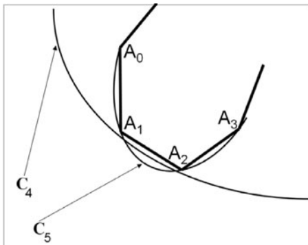
(a) Inscribed polygon A_0A_1A_2A_3 \dots may produce false-positive containment test
