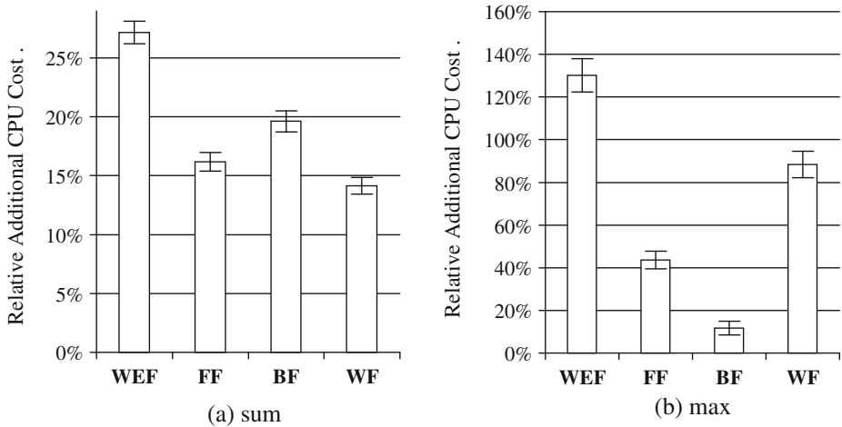
Fig. 16 Performance of different elimination order policies (99% confidence level)
