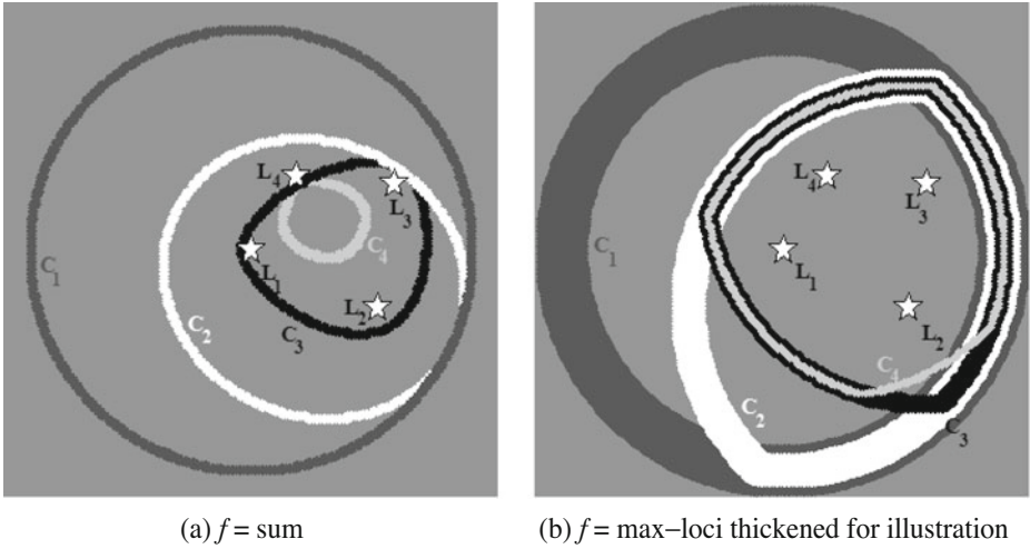
Fig. 9 Use of the loci of aggregate distance functions in computing the thresholds. C_i represents E(f, i) = R_i
