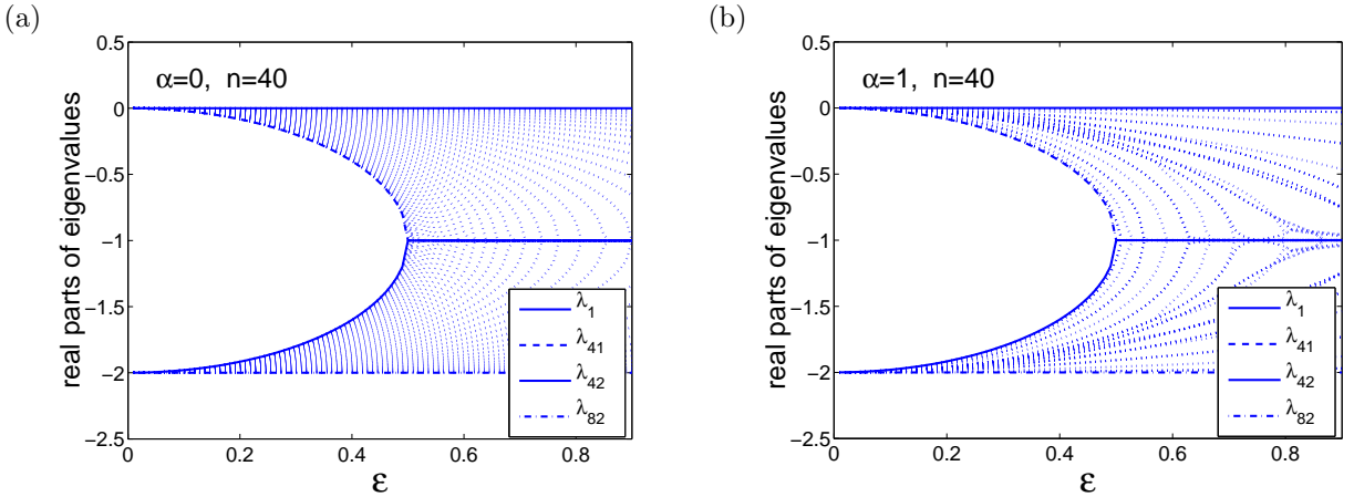
Figure 7: (a) Graph of real parts of eigenvalues of matrix \mathcal{B} for n = 40 and no signal gradient in the environment, i.e. , S'_0 = S'_1 = \dots S'_n = 0 . The eigenvalues are real for \varepsilon \in [0, 0.5] and there is a spectral gap between \lambda_{41} and \lambda_{42} . (b) Graph of real parts of eigenvalues of matrix \mathcal{B} for signal given by (3.27) with \alpha = 1 and for n = 40 .
