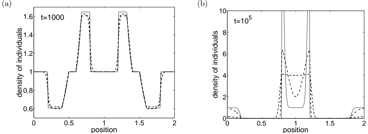
Figure 11: (a) Density of individuals for s = 0.0001 and \alpha = 1 at time t = 1000 . We plot the solution of (NJ) given by accurate numerical method (solid line), the solution obtained by projective algorithm (P_k^M-1) - (P_k^M-3) for (4.13) with (4.22), k = 1 and M = 198 , i.e., with \mathcal{G} = 100 (dashed line). We also plot the solution obtained by projective algorithm (P_k^M-1) - (P_k^M-3) for (4.13) with (4.24), k = 1 and M = 18 , i.e., with \mathcal{G} = 10 (dot-dashed line). In all computations, we use (4.19) and (4.23). (b) The same plots as in (a) for time t = 10^5 .
