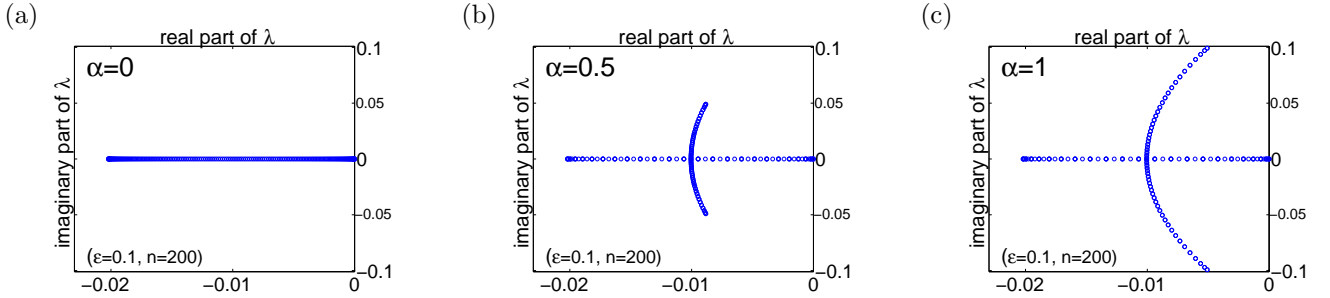
Figure 8: A plot of ‘‘slow’’ eigenvalues of matrix \mathcal{B} for n = 200 and \varepsilon = 0.1 . We plotted only eigenvalues close to zero for different strength of the signal \alpha from (3.27), namely: (a) \alpha = 0 , (b) \alpha = 0.5 and (c) \alpha = 1 .
