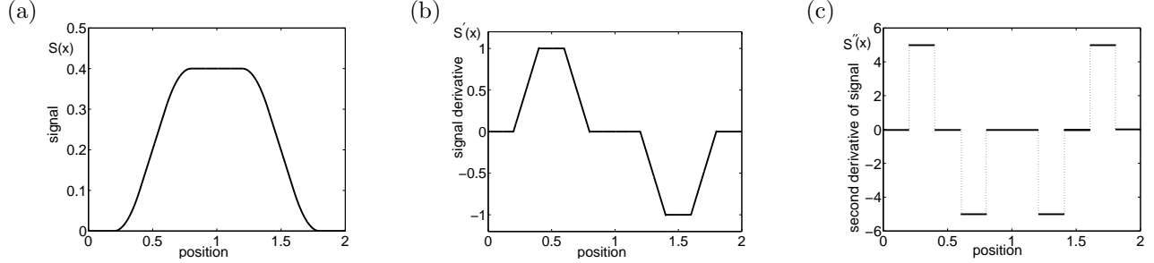
Figure 3: (a) Graph of “hat-profile” signal function \bar{S}(x) . (b) Graph of \bar{S}'(x) . (c) Graph of \bar{S}''(x) .
