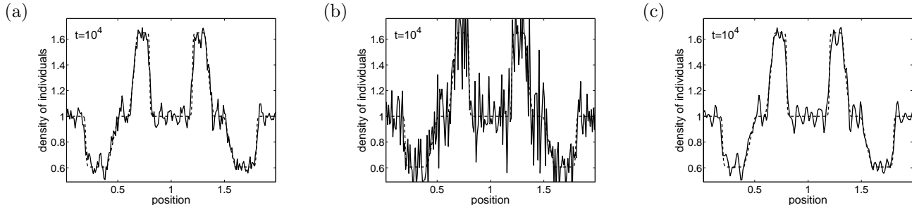
Figure 14: Plots of the density of individuals at time t = 10^4 for the same cumulative distribution function as in Figure 13. We choose different formulas for computing discretized density, namely: (a) formula (5.9); (b) formula (5.10); (c) formula (5.11). We also plot the solution of the corresponding macroscopic moment equations (dashed line).
