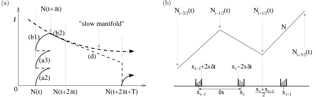
Figure 12: (a) Schematic of steps (a1) – (d) of the coarse integration algorithm. Monte Carlo simulation is denoted by solid lines. Dashed lines denote relatively fast steps, i.e., resetting the values of density to N(t) in steps (a2) and (a3) and the projective step (d). The dot-dashed line represents the slow manifold of the system. We assume that the slow manifold can be accurately parametrized by density. (b) Schematic of three macroscopic mesh points x_{i-1} , x_i and x_{i+1} and kMC computational domains around them. Only particles close to the meshpoints need be considered; the remaining particles will not leave/enter the interval [0, x_i] during steps (a1) – (b2) and consequently, they do not have to be simulated. At the top, is the (piecewise linear) estimated density profile which is used in step (a1). We place particles in the small computational domains such that their number is consistent with this density profile.
