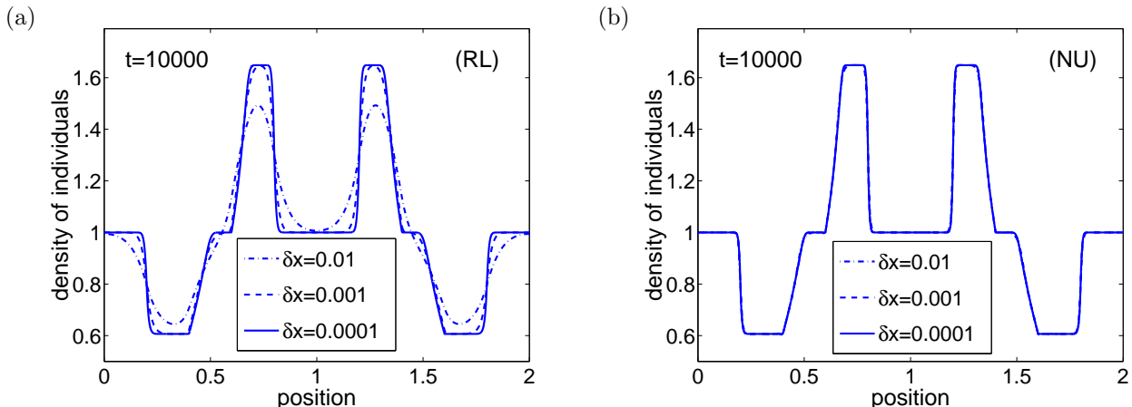
Figure 9: (a) Graph of a solution of (RL) given by \dot{w} = \mathcal{A}w at time t = 10^4 for different choices of \delta x . We used s = 0.0001 , signal given by (3.27) with \alpha = 0.1 , \delta t given by (4.19) and initial conditions (4.23). Consequently, \delta x = 0.01 , \delta x = 0.001 and \delta x = 0.0001 correspond to \varepsilon = 0.01 , \varepsilon = 0.1 , and \varepsilon = 1 , respectively. (b) Graph of a solution of (NU) given by \dot{z} = \mathcal{B}z at time t = 10^4 for different choices of \delta x . The parameters are the same as in (a).
