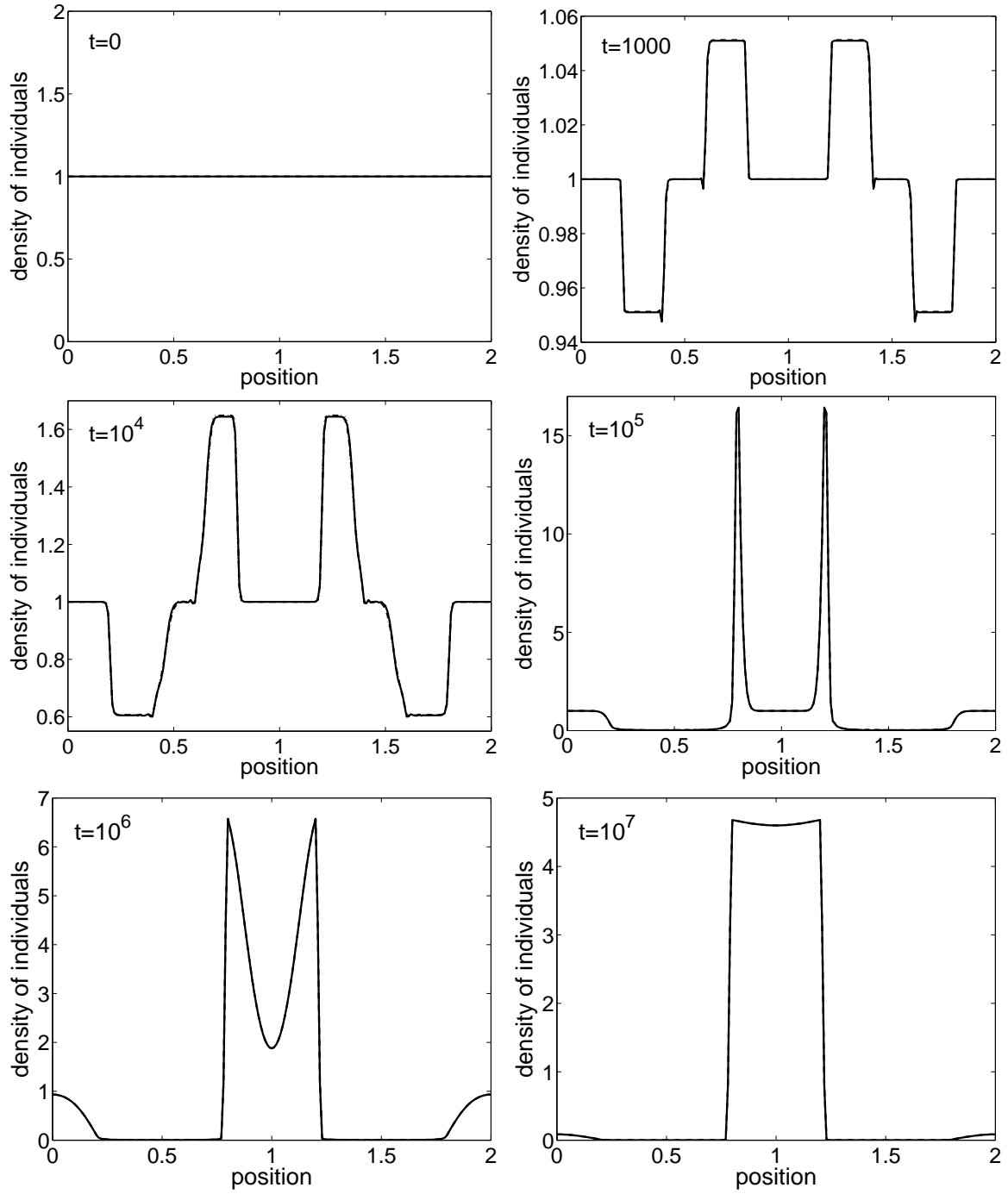
Figure 10: The time evolution of the density of individuals for s = 0.0001 and \alpha = 0.1 . We plot the solution of the system (4.16) (dashed line) and the solution obtained by the projective algorithm (P_k^M - 1) - (P_k^M - 3) for (4.16) with k = 1 and M = 398 (solid line). The gain \mathcal{G} is 200. We use (4.22), (4.19) and (4.23).
