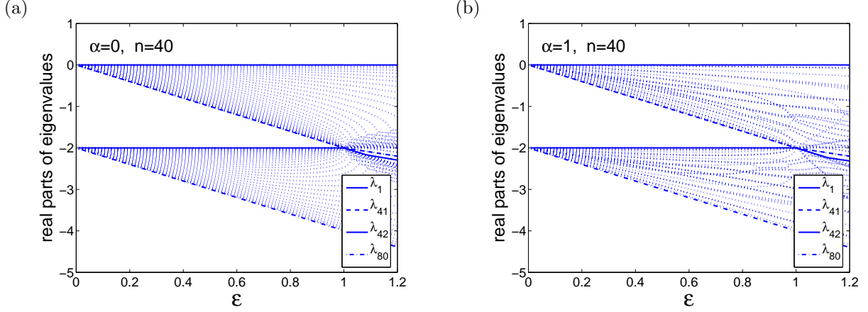
Figure 6: (a) Graph of real parts of eigenvalues of matrix \mathcal{A} for n = 40 and no signal gradient in the environment, i.e. , S'_0 = S'_1 = \dots S'_n = 0 . The eigenvalues are real for \varepsilon \in [0, 1] and there is a spectral gap between \lambda_{41} and \lambda_{42} . (b) Graph of real parts of eigenvalues of matrix \mathcal{A} for signal given by (3.27) with \alpha = 1 and for n = 40 .
