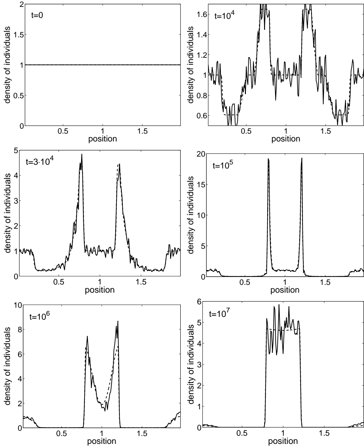
Figure 13: The time evolution of the density of individuals for (5.1), (5.5), \alpha = 0.1 and initial conditions (4.23). We plot the density given by coarse integration (a1) – (d) and obtained by formula (5.8) from the computed cumulative density function C(t) (solid line). Here we have gain \mathcal{G} = 1250 . We also plot the solution of the corresponding macroscopic moment equations (dashed line).
