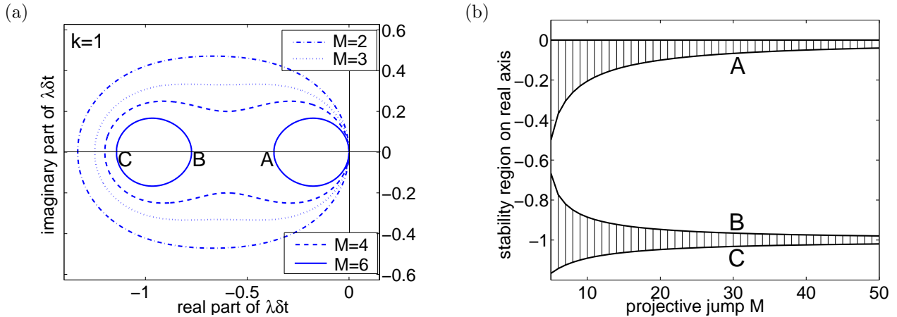
Figure 5: (a) The regions of absolute stability of P_k^M methods for k = 1 and M = 2 (dot-dashed line), M = 3 (dotted line), M = 4 (dashed line) and M = 6 (solid line). (b) Intersection of stability region from part (a) with real axis plotted as a function of M . The equations for boundary curves A(M) , B(M) and C(M) are given in Lemma 2.
