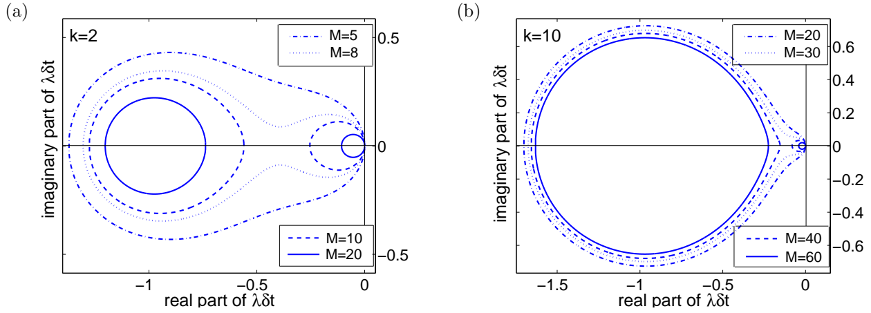
Figure 4: (a) The regions of absolute stability of P_k^M methods for k = 2 and M = 5 (dot-dashed line), M = 8 (dotted line), M = 10 (dashed line) and M = 20 (solid line). (b) The regions of absolute stability of P_k^M methods for k = 10 and M = 20 (dot-dashed line), M = 30 (dotted line), M = 40 (dashed line) and M = 60 (solid line).
