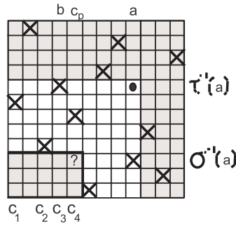
FIGURE 8. For \tau to be greater than \sigma in Ding order, cell (\sigma^{-1}(a), c_p) must exist in board \lambda . The X's are rooks in \sigma and the dot is a rook in \tau .
