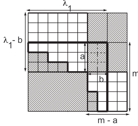
FIGURE 4. R_\lambda^\omega \subset S_{m-a} \times S_{\lambda_1-b} \subset S_{\lambda_1+m-\omega} where \omega = a + b and a and b are defined below.
