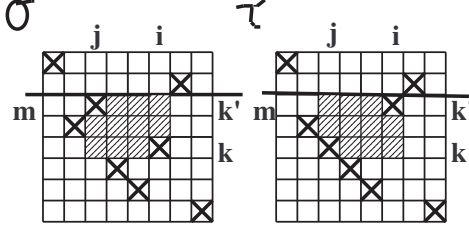
FIGURE 6. Increasing a single i is a swap.
