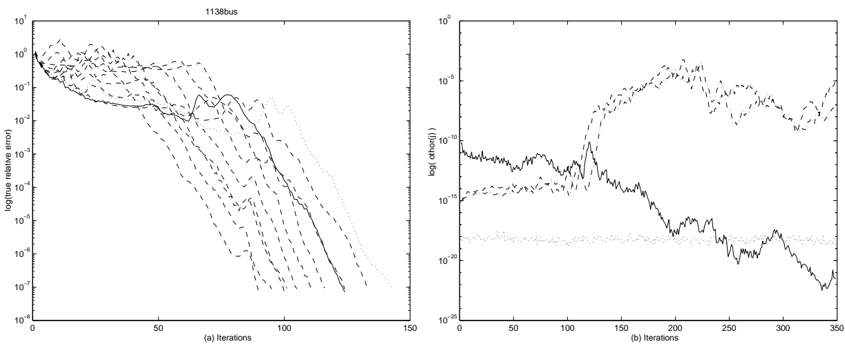
Figure 2: (a) Convergence curves for matrix 1138bus. (b) dashed: system 2 solved by AugCG; dashdot: system 5 solved by Deflated-CG; solid: system 2 solved by AugCG with correction; dotted: system 5 solved by Deflated-CG with correction.
