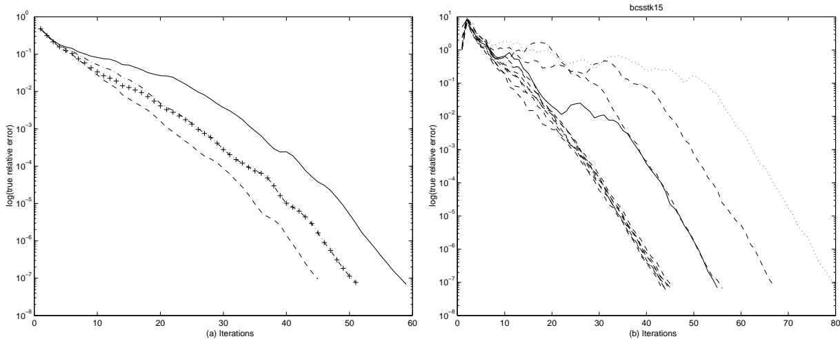
Figure 1: (a) Illustration of the analysis in Section 5. (b) Convergence curves for matrix BCSSTK15.
