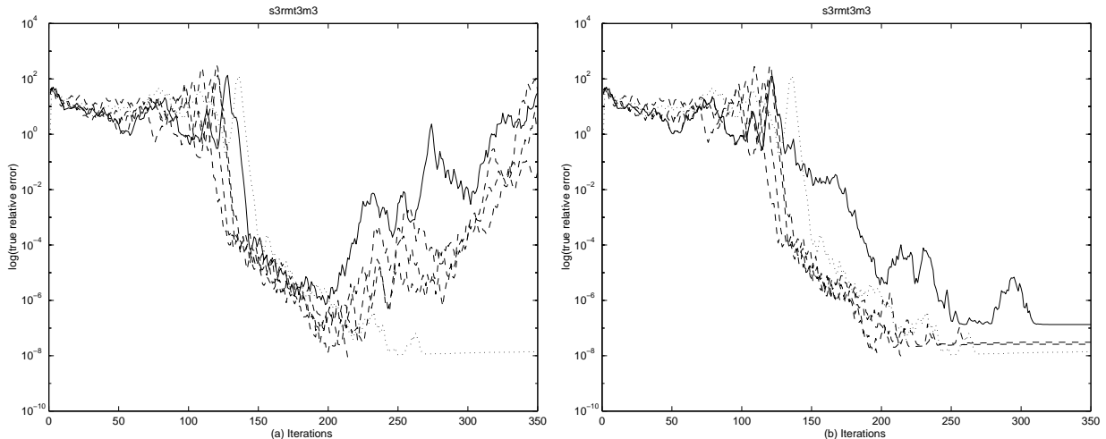
Figure 3: (a) Convergence curves for matrix S3RMT3M3. (b) Convergence curves with correction of r_j for matrix S3RMT3M3.
