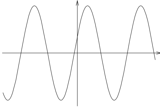
Figure 2. The graph of A \cos(ct - \varphi)
