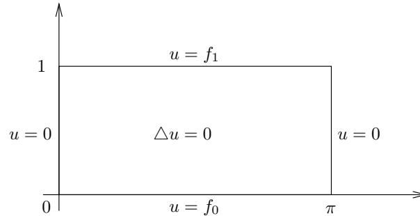
Figure 11. Dirichlet problem in a rectangle
