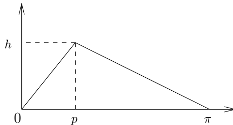
Figure 8. Initial position of a plucked string
