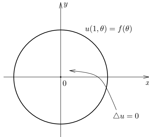
Figure 10. The Dirichlet problem for the disc
