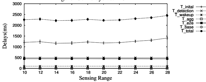
Figure 21: Delays vs. Sensing Range
