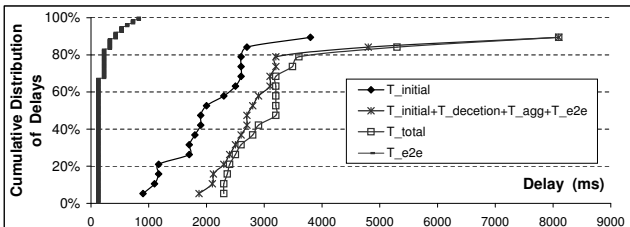
Figure 10: Various Delays Measurements from Field Test
