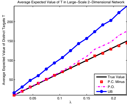
Figure 14. Average Ex-pected Count vs. \lambda
