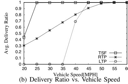
Figure 9. Impact of Vehicle Speed \mu_v
