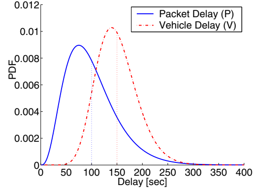
Figure 2. Packet Delay Distribution and Vehicle Delay Distribution
