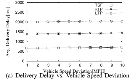
(a) Delivery Delay vs. Vehicle Speed Deviation
