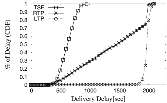
Figure 7. CDF Comparison for Delivery Delay
