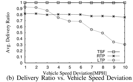
Figure 10. Impact of Vehicle Speed Deviation \sigma_v
