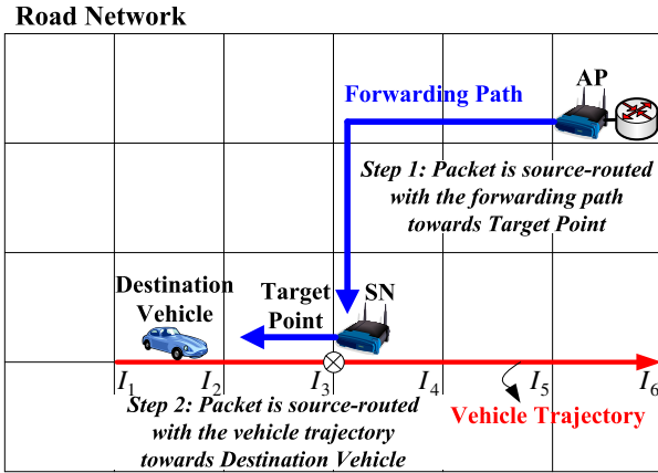
Figure 6. TSF Forwarding Protocol
