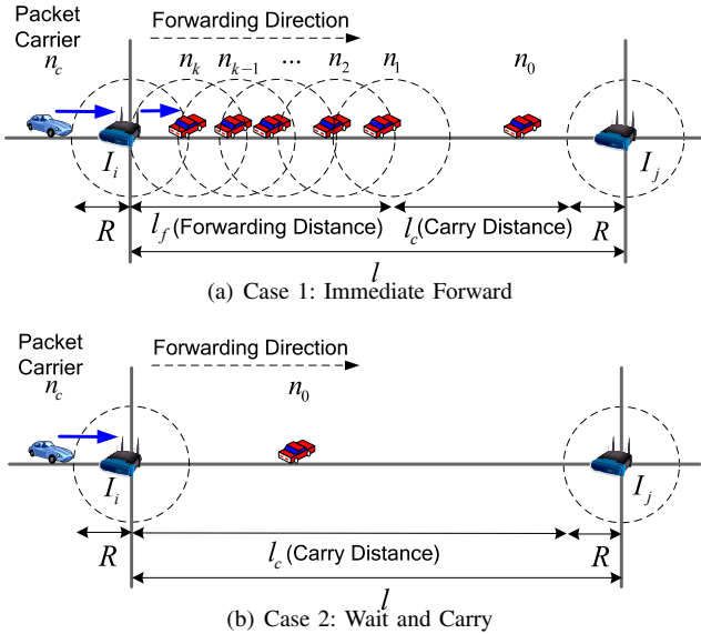
Figure 3. Link Delay Modeling for Road Segment
