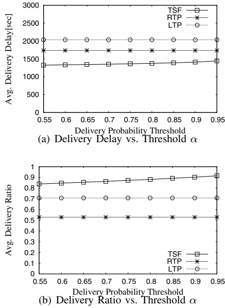
Figure 11. Impact of Delivery Probability Threshold \alpha
