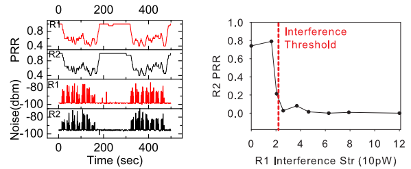
Figure 2: Cross-network interference; (a) two receivers' PRR and the corresponding noise level. Both receivers' PRR decreases when the noise is introduced by the microwave oven. (b) R2's PRR under R1's interference strength. We can tell R2's PRR from R1's interference strength – R2's PRR decreases when R1's interference is above a certain level.
