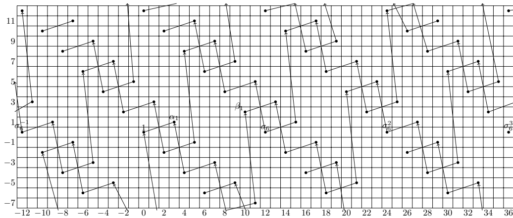
Figure 1: The Tate E_2 -term
