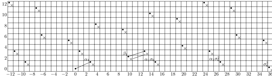
Figure 2: The E_6 -page of the homotopy fixed points
