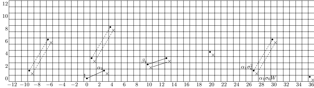
Figure 3: The E_\infty -page of the homotopy fixed points
