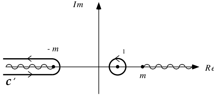
Figure 2: The deformed integration contour C' used in Eq. (3.3).
