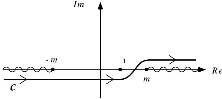
Figure 1: The contour \mathcal{C} in the complex \omega plane in Eq. (3.3). The continuum states appear as the two cuts along the real axis with branch points at \pm m (wiggly lines), and the bound state is the pole at \omega_1 .
