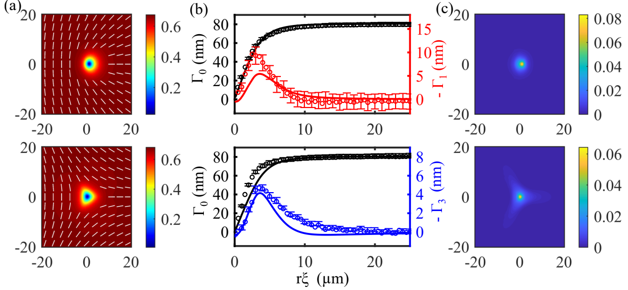
FIG. 2. (a,b) Optical retardance \Gamma and (c) biaxiality P for a +1/2 disclination (top) and -1/2 (bottom). Solid lines in (b) are solutions to the molecular field theory, dots are the experimental data points in Ref. [28].
