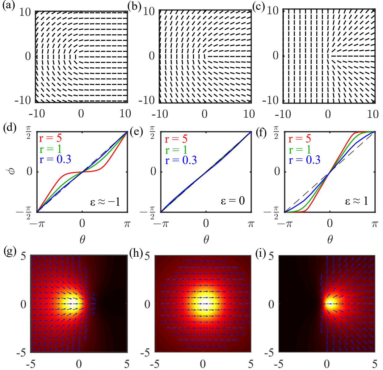
FIG. 1. (a-c) Director configuration, (d-f) director angle \phi versus polar angle \theta for three radial distances from the core, and (g-i) disclination polarization \nabla \cdot \mathbf{Q} . Left: \epsilon \approx -1 , center: \epsilon = 0 , and right: \epsilon \approx 1 . For \epsilon \neq 0 the polarization is nonuniform and exhibits contractile or extensile vector flows.
